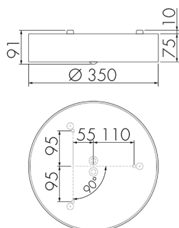
Abmessungen in mm
