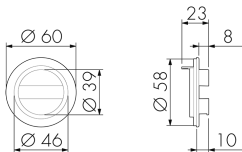
Abmessungen in mm
