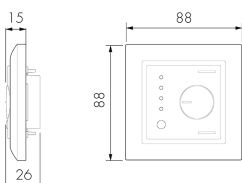
Abmessungen in mm
