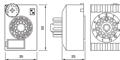
fig. 2. Dimensions (mm)
