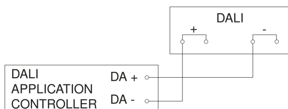
Circuit diagram
