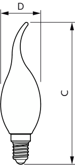
MAS LEDCandleDT3.4-40W E14927 BA35CL G
