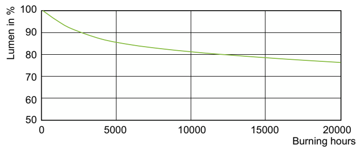
Lumen Maintenance Diagram - MASTERColour CDM-T MW eco 360W/842
