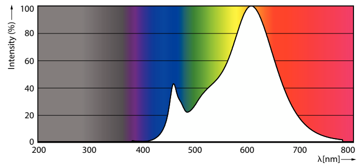
Spectral Power Distribution Colour - CorePro LEDcapsuleLV 2.7-28W G4 827
