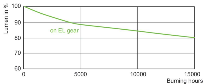
Lumen Maintenance Diagram - MASTERC CDM-TC Elite 70W/930 G8.5
