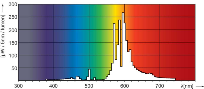
Spectral Power Distribution Colour – MASTER SON PIA Plus 70W E27
