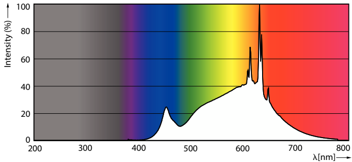
Spectral Power Distribution Colour - MAS LEDspotLV D 7.5-50W 930 MR16 36D
