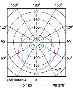
Light Distribution Diagram - CorePro LEDtube HF 600mm HE 7.1W 840T5
