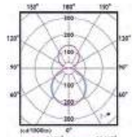
SP533P, opal
