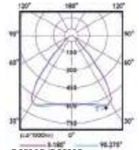
RC530B/RC532B, BAP-tauglich
