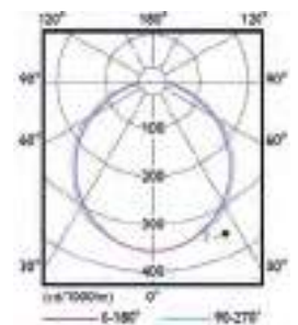
RC531B/RC533B, opal
