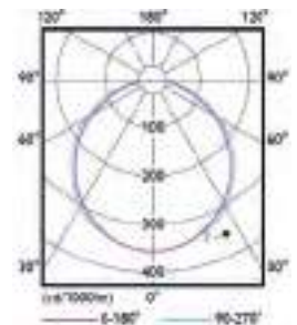
SM541C, opal
