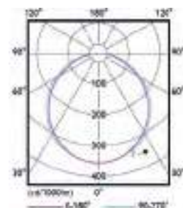
SM531C, opale
