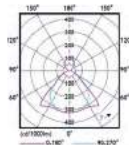
SP482P, direct-indirect
