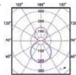
SP533P, opale
