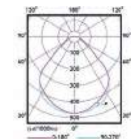
SP402P, direct, carrée
