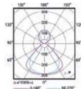
SP402P, direct-indirect
