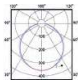
RC531B/RC533B, opale
