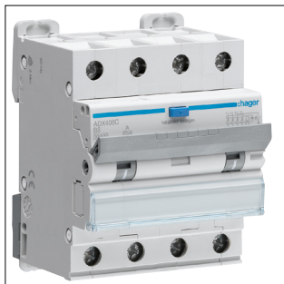
ADX406C
