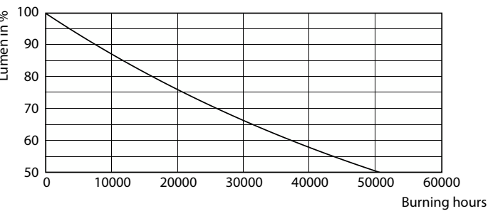
Lumen Maintenance Diagram - MAS LED SPOT VLE D 7.5-50W MR16 940 36D
