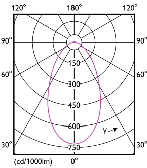
Light Distribution Diagram - TForce LED HPI UN 140W E40 840 NB
