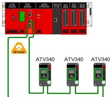
Architecture CIP Safety
