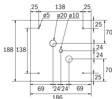
Drilling distances AWWK
