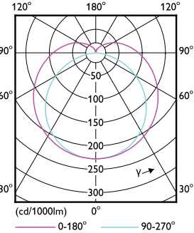
Light Distribution Diagram - MAS LEDtube 1500mm UE 20W 865 T8
