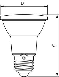
MAS LEDspot VLE D 6-50W 940 PAR20 25D
