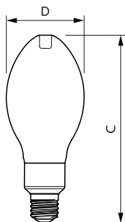
MAS LED HPL M 3Klm 19W 840 E27 FR G
