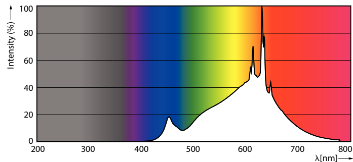
Spectral Power Distribution Colour - MAS LED spot VLE D 5.8-35W MR16 927 60D
