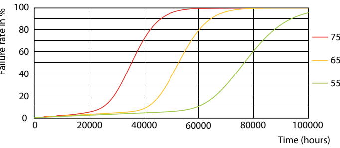
LEDtube-75K-5575-FailureRate-LED
