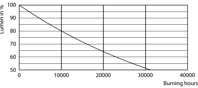
Lumen Maintenance Diagram - MAS VLE LEDBulb D5.9-60W E27 927 G120CLG
