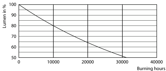
Lumen Maintenance Diagram - MAS VLE LEDBulbD4-25WE27 G93GOLD SP
