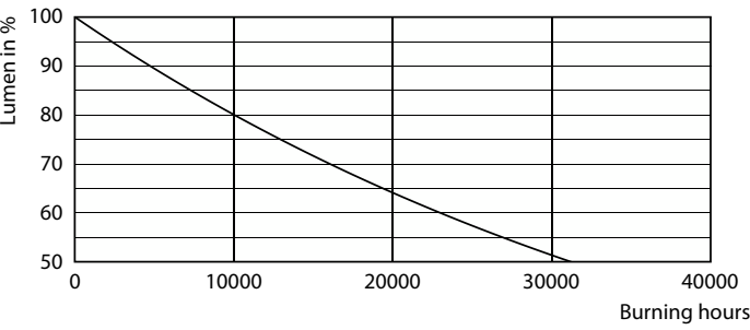
Lumen Maintenance Diagram - CorePro candle ND 7-60W E14 827 B38 FR
