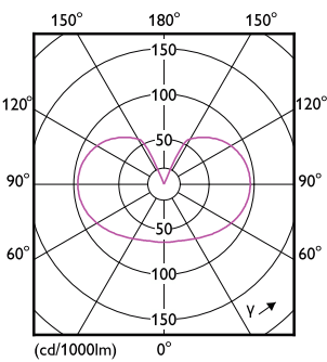
Light Distribution Diagram - CorePro LEDBulbND10.5-100W E27A60 827FRG
