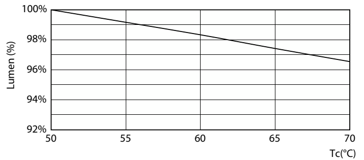
Lumen Maintenance Diagram - CorePro LEDtube UN 1200mm UO 15.5W830 T8
