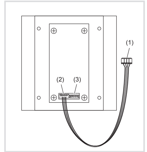
Figure 1: Rear view
