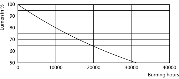
Lumen Maintenance Diagram - MAS VLE LEDBulbD4-25W E27 A60 GOLD SP G
