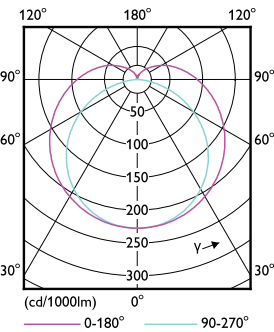
Light Distribution Diagram - MAS LEDtube 1200mm UE 13.5W 865 T8
