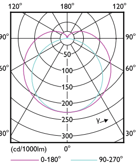
Light Distribution Diagram - MAS LEDtube 1500mm HO 16.7W 865 T8 EELB
